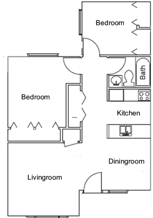
2- Bedroom Flat Floor Plan
